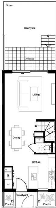
GROUND FLOOR
